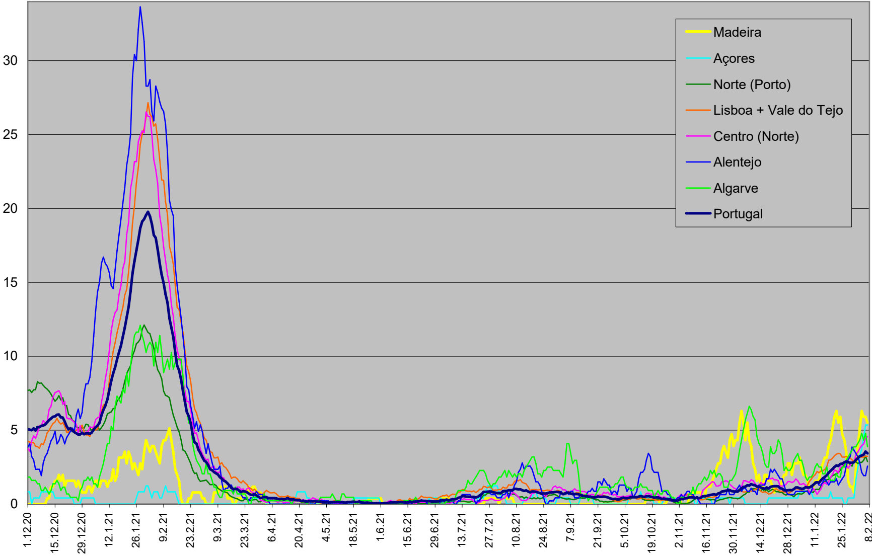
Covid-19 in Portugal: Fatalities (7day incidence per 100.000) (Source: DGS Bulletins)
